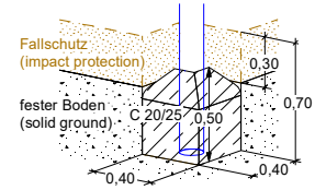
Alternativ: Fundament flach/kantig (Alternative: Foundations plain/edged)
